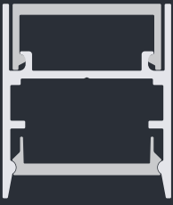
7CCE Cube 26x34 26 x 33.9 mm
