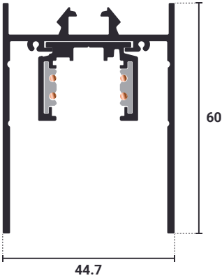
Misure (mm) / Measurements (mm)
