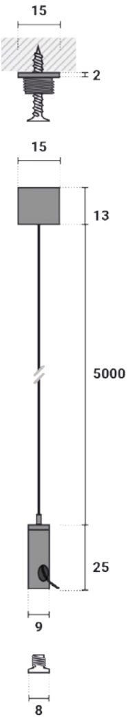
Misure (mm) / Measurements (mm)
