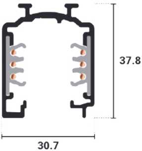
Misure (mm) / Measurements (mm)
