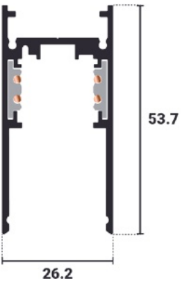
Misure (mm) / Measurements (mm)
