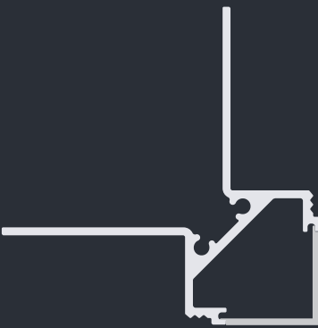
7CEC Spigolo 47.8 x 47.8 mm
