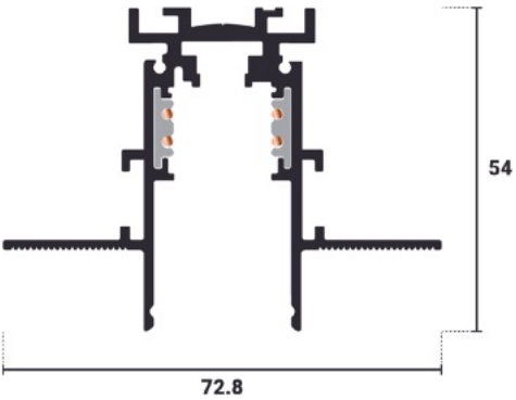
Misure (mm) / Measurements (mm)
