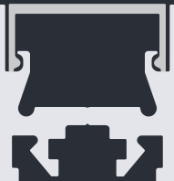
5DC0 Lynn 26x26 26.2 x 26.2 mm
