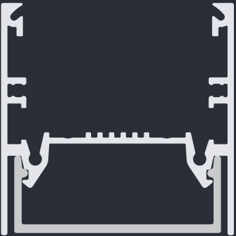
7D90 Modulo Quadro 43.5 x 43.5 mm
