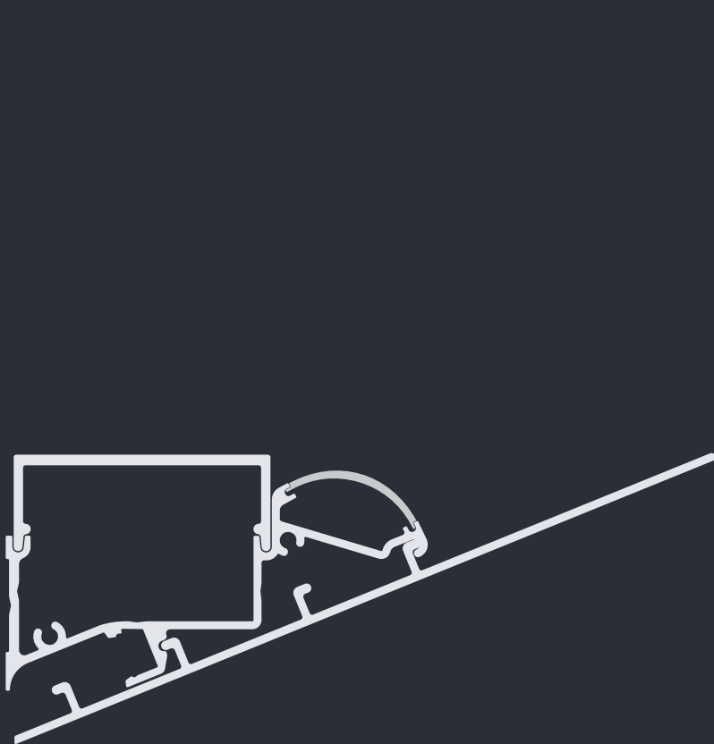
7D00 Aria 105.6 x 43.6 mm
